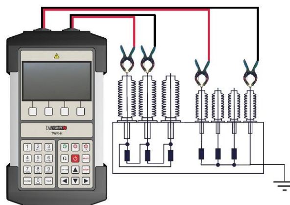
Connecting TWR-H to a three-phase distribution transformer
